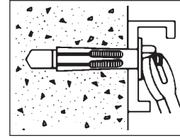
TIGHTEN
