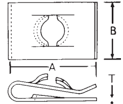
'U' Types
