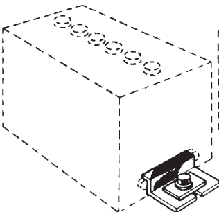
Card No. 570-509 Universal end type for base mount battery groups 22NF, 27F and 29NF.
