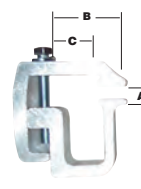
APIKH1U A= 0" à / to 7/8" B= 1 3/4" C= 1"
