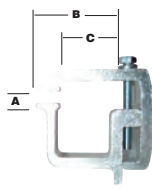
APIAC103U A= 0" à / to 1 3/8" B= 2 1/2" C= 1 3/4"
